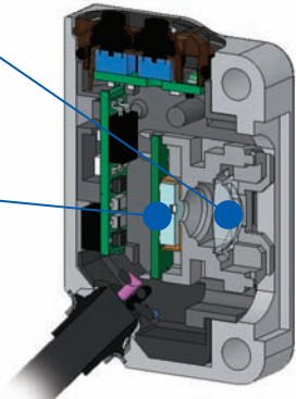
Cross Section
