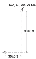
Mounting Holes
