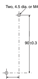
Mounting Holes
