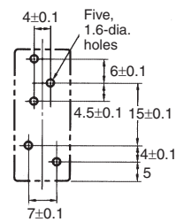
Mounting Holes (Bottom View)
