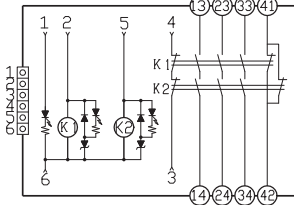
G9SA-EX301型
