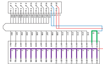
XW2K-20G-O16B-OUT
