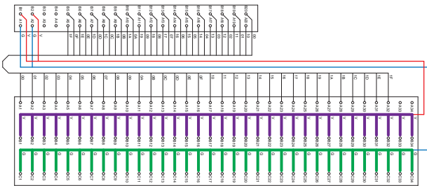
XW2K-40G-M32-IN
